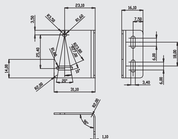
OS12 series mounting bracket EOS12DF-2
